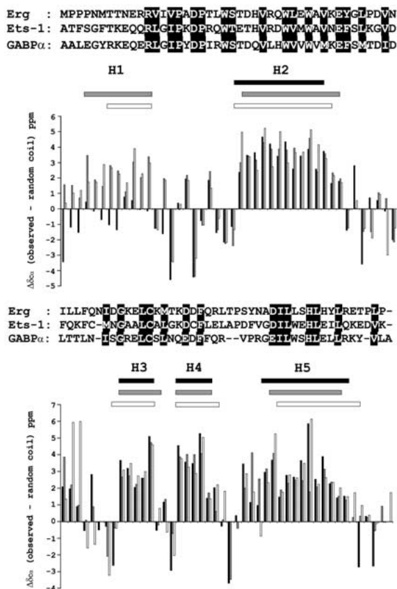
Figure 1. ^{13}\text{C}^\alpha secondary chemical shifts for Erg (108–201) (black), Ets-1 (29–138) (gray) and GABP \alpha (168–254) (white) calculated using random coil reference values from Wishart and Sykes (1994). Also illustrated is a sequence alignment (with highly conserved residues boxed), along with horizontal bars showing the locations of helical regions defined by chemical shift, ^3J_{\text{HN-H}\alpha} coupling, and in the case of Ets-1 (29–138) , tertiary structural analysis. Erg shares the core four \alpha -helices (H2–H5) common to all PNT/SAM structures, yet clearly lacks the N-terminal helix (H1) found in Ets-1 and GABP \alpha .
